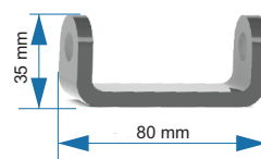
Cavalete Lateral 10.02.012
