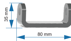
Cavalete Lateral 10.02.012
