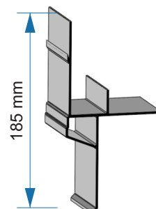
Saia 185 Tubular 50.04.004
