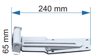
Cj. Dobradiça Inox 240 mm Cod - 99.00.818 270 mm Cod - 99.00.418 300 mm Cod - 16.00.006
