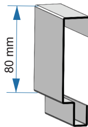
Coluna Q.Lat. 80mm 99.00.026
