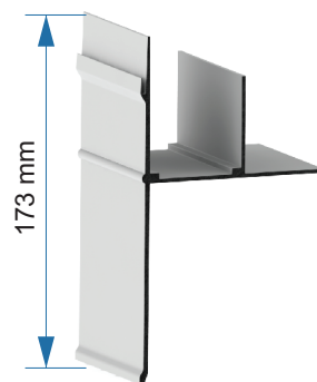
Saia 173 50.13.003
