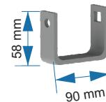
Cavalete Lat. 10.04.012
