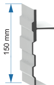
Saia Recrosul 150 50.11.001
